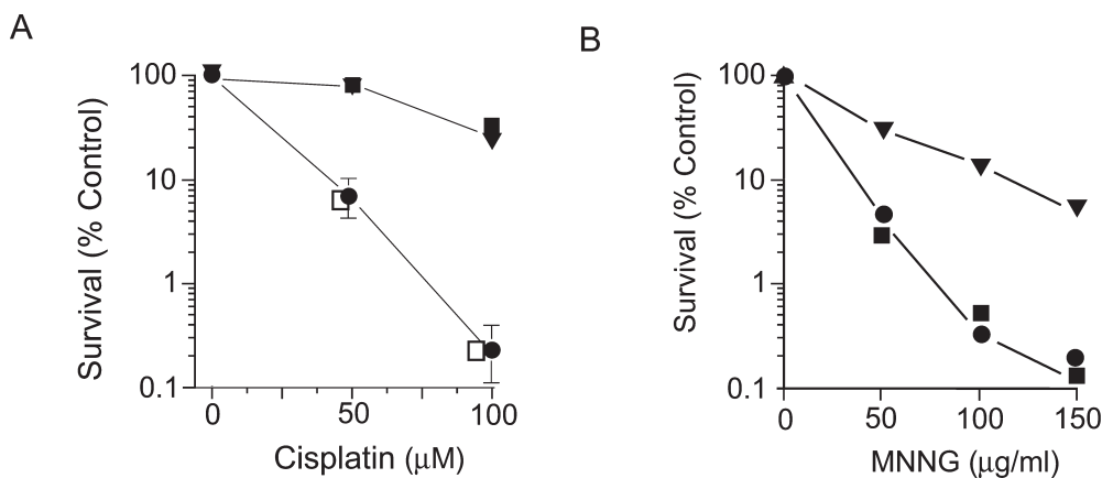
Figure 2. Survival of cells exposed to cisplatin and MNNG. Cell survival of strain GM5556 ( \Delta dam-16::Kan mutS::Tn10 ) containing plasmids with mutS + (closed circles), mutS Δ680 (inverted triangles), and mutS Δ800 (closed squares) after exposure to cisplatin (A) and MNNG (B). The open squares in (A) represent the survival of GM3819 ( \Delta dam-16::Kan mutS ) with the mutS Δ800 plasmid.
