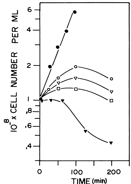
FIG. 3. Effect of TL on cell viability. Exponentially growing cultures of E. coli 15 TAU (GK 117) growing in NB and E. coli K-12 (GK 19) growing in medium E + glycerol were exposed to TL at zero time at 5 (○), 20 (▽), and 50 (□) \mu\text{g/ml} . (▼) represents GK 19 treated with 20 \mu\text{g} of TL/ml. Closed circles (●) represent untreated control of strain GK 117.
