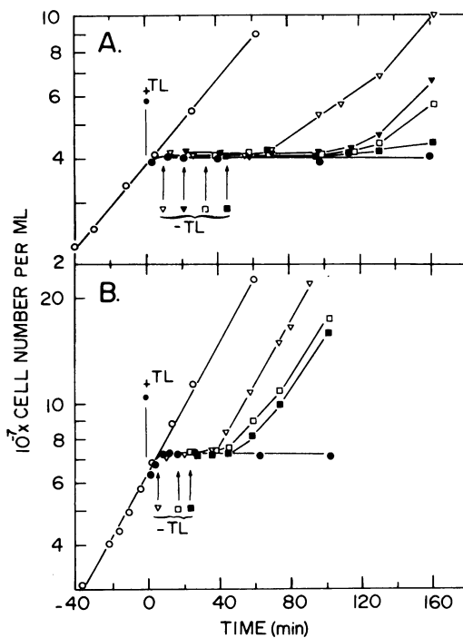
FIG. 5. Effect of growth media on recovery of cell division. Cells of E. coli K-12 (GK 19) were grown in the absence (A) or presence (B) of Casamino Acids in medium E + glucose (○) and treated with 20 μg of TL per ml (●) at zero time. At times equivalent to the 0.25 (▽), 0.50 (▼), 0.75 (□), and 1.0 (■) generation time, samples of TL-treated cells were removed and washed free of the drug. Recovery of cell division was monitored with a Coulter counter.
