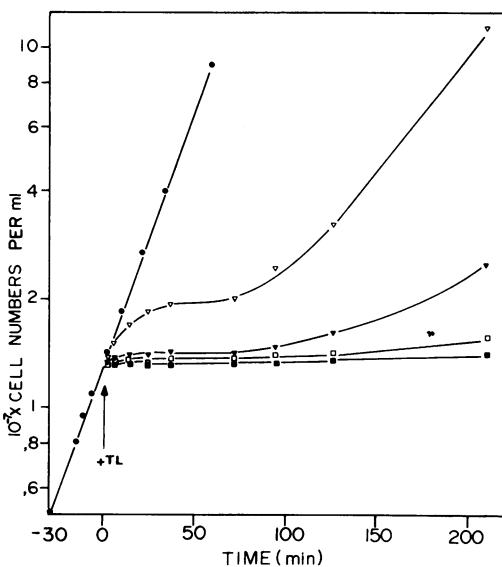
FIG. 1. Effect of thiolutin on cell multiplication in E. coli 15 TAU. Exponentially growing cells of strain GK 117 in medium A + E + glucose were exposed to TL at concentrations of 1, 5, 20, and 50 \mu\text{g/ml} at time zero (arrow). The cell density at the time of addition of TL was 5 \times 10^7 cells/ml. Cell counts are plotted versus incubation time.
