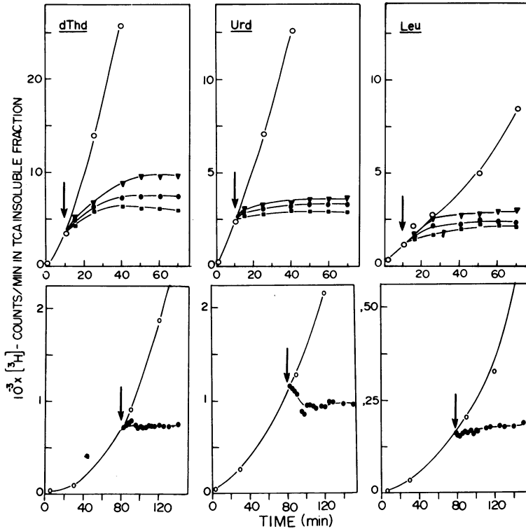
FIG. 4. Effect of TL on macromolecular synthesis in E. coli . Incorporation of radioactive precursors of DNA, RNA, and protein synthesis, thymidine (10 mM), uridine (10 mM), and leucine (20 mM) into cells of GK 255 (upper panel) and GK 117 (lower panel) are shown. TL at concentrations of 5 (▼), 20 (●), or 50 (■) µg/ml was added as indicated by the arrow. Open circles represent control (dimethyl sulfoxide-treated) cells.
