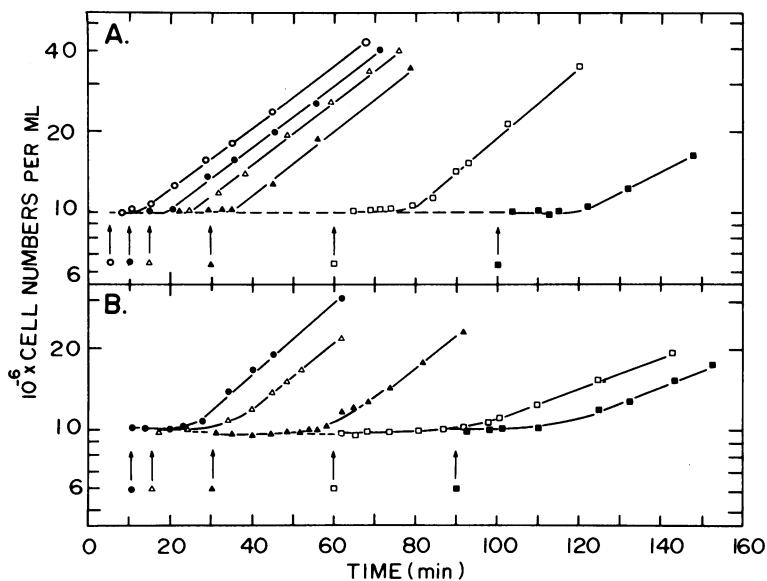
FIG. 6. Recovery of cell division after treatment with different concentrations of TL. Exponentially growing cultures of GK 117 (in medium A + E) were treated with (A) 5 or (B) 20 \mu\text{g} of TL per ml at zero time. After a period of treatment indicated in each graph by the arrows, the cultures were washed free of TL and incubation was resumed in drug-free medium. Cell counts were monitored for each case and are plotted versus incubation time.
