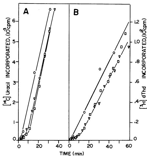
FIG. 7. Recovery of macromolecular synthesis after treatment with TL. Cells of E. coli K-12 (GK 255) growing in medium A + glucose at 37 C were treated with 20 \mu\text{g} of TL per ml. Five ( \nabla ) and 40 min ( \square ) after the treatment began, cells were washed free of the drug and incubated in drug-free medium. Incorporation of [ ^3\text{H} ]thymidine (A) and [ ^{14}\text{C} ]uracil (B) as shown as a function of time of incubation in drug-free medium. Unlabeled thymidine and uracil were each added at 10 \mu\text{M}/\text{ml} . Circles represent controls subjected to the same procedure but without TL.
