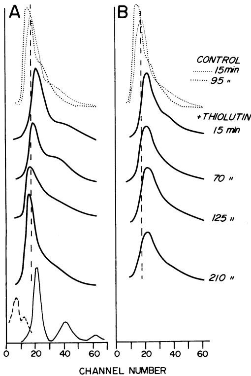
FIG. 2. Effect of TL on cell growth. Profiles of cell volume distribution for GK 117 treated with TL at 1 (A) and 20 (B) \mu\text{g/ml} were obtained from plots of the pulse height analysis of cell samples taken after addition of drug at times indicated in the right-hand side. Untreated controls are shown at the top. The vertical dashed line in each panel indicates the mode at 0 min for cell size distributions. In each case, the total number of cells under the profile were kept at a constant cell number of 4.00 \pm 0.02 \times 10^7 cells/ml. The ordinate represents the cell numbers per channel, and the abscissa represents the pulse height analyzer channel number (0 to 200). The lower left distribution (A) is calibration with polystyrene latex microspheres 0.8 \mu\text{m} in diameter (volume, 0.27 \mu\text{m}^3 ) in broken lines and 1.099 \mu\text{m} in diameter (volume, 0.69 \mu\text{m}^3 ) in solid line. The peaks represent the volumes of one, two, or three microspheres.
