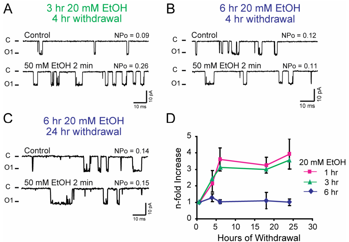
Figure 2. Persistence of rapid tolerance is a function of ethanol exposure time. BK channel activity ( NP_o ) before and after exposure to 50 mM EtOH in a cell-attached patch from striatal neurons which were (A) pre-exposed to 20 mM EtOH for 3 hr and ethanol withdrawn for 4 hr, (B) pre-exposed to 20 mM EtOH for 6 hr and ethanol withdrawn for 4 hr, or (C) pre-exposed to 20 mM EtOH for 6 hr and ethanol withdrawn for 24 hr. All traces were recorded at a holding potential of -60 mV. C and O represent the closed and open state, respectively. (D) Scatter plot of the n-fold increase in BK channel activity after exposure to 50 mM EtOH in striatal neurons pre-exposed to 20 mM EtOH for 1, 3, or 6 hr (pink, green, and blue, respectively) followed by various periods of withdrawal.
