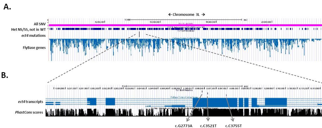
Figure 3. Mutation density on chromosome 3L in screen (N = 3). (A) Screenshot of chromosome 3L with custom tracks in the UCSC genome browser. The pink line displays all SNVs on chromosome 3L that were detected in this screen. The navy line displays all heterozygous non-synonymous and splice-site SNVs on chromosome 3L not present in the wild-type fly. (B) Screen shot of ect4/dSarm with custom track displaying the location and conservation of the three ect4 mutations.
