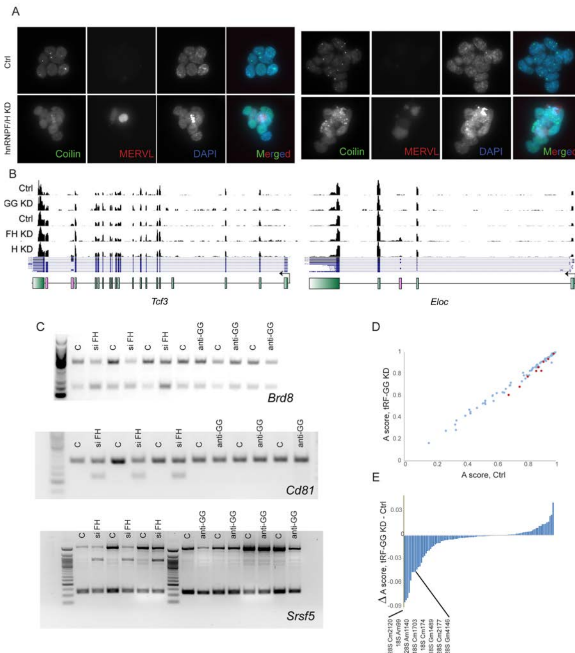
Figure 3.10. Effects of hnRNPF/H on Cajal bodies and MERVL expression.
