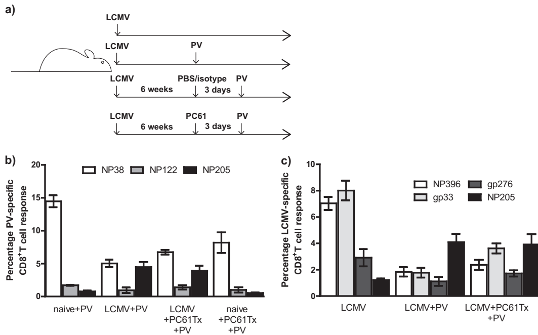
FIG 6 PC61 treatment (anti-CD25) in LCMV-immune mice prior to PV infection does not affect reactivation and immunodomination by cross-reactive NP205-specific memory CD8 + T cells. (a) Experimental setup of sequential LCMV and PV (LCMV +PV) infections with PC61 treatment. Three days prior to PV infection, LCMV-immune (LCMV) mice were treated with PBS/isotype or PC61 (anti-CD25) (LCMV +PC61) and compared to PBS/isotype-treated naive mice. LCMV and PV epitope-specific responses were determined using peptide stimulation in an intracellular cytokine assay at day 8 post-PV infection. (b) Percentage of PV-specific CD8 + T-cell responses (NP38, NP205, and NP122) was determined in spleens at day 8 post-PV infection in PC61-treated or nontreated LCMV-immune mice. (c) Percentage of LCMV-specific CD8 + T-cell responses (NP396, GP33, GP276, or NP205) was determined in spleens at day 8 post-LCMV infection in PC61-treated or nontreated LCMV-immune mice.
